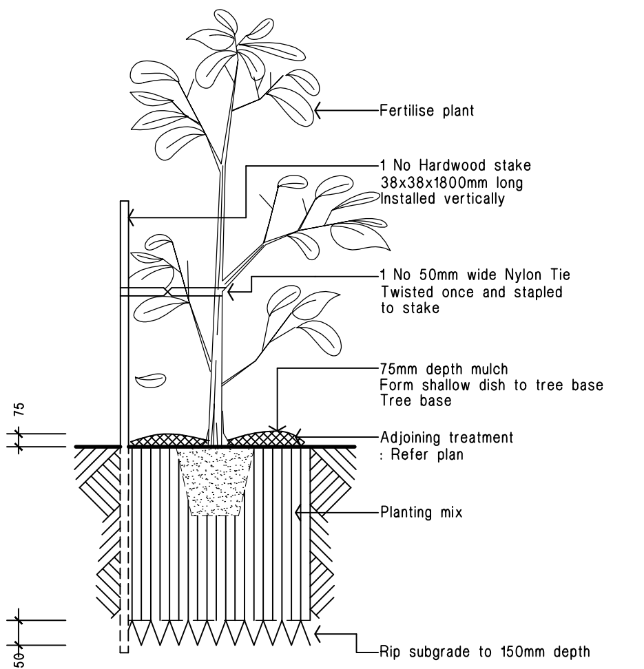
45 litre Tree planting Detail. Not To Scale.
