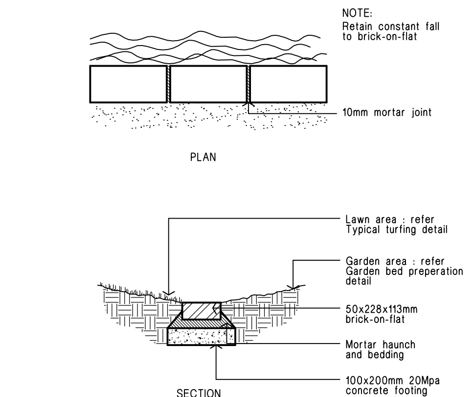
Brick garden edge Detail. Not To Scale.
